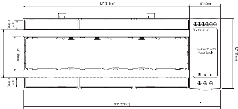
Figure 1 - Top View
