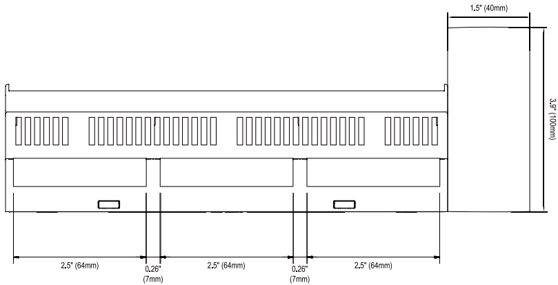
Figure 3 - Front view
