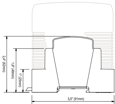
Figure 2 - Side View
